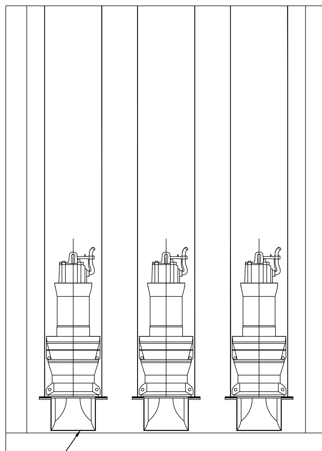
SECTION VIEW C-C
