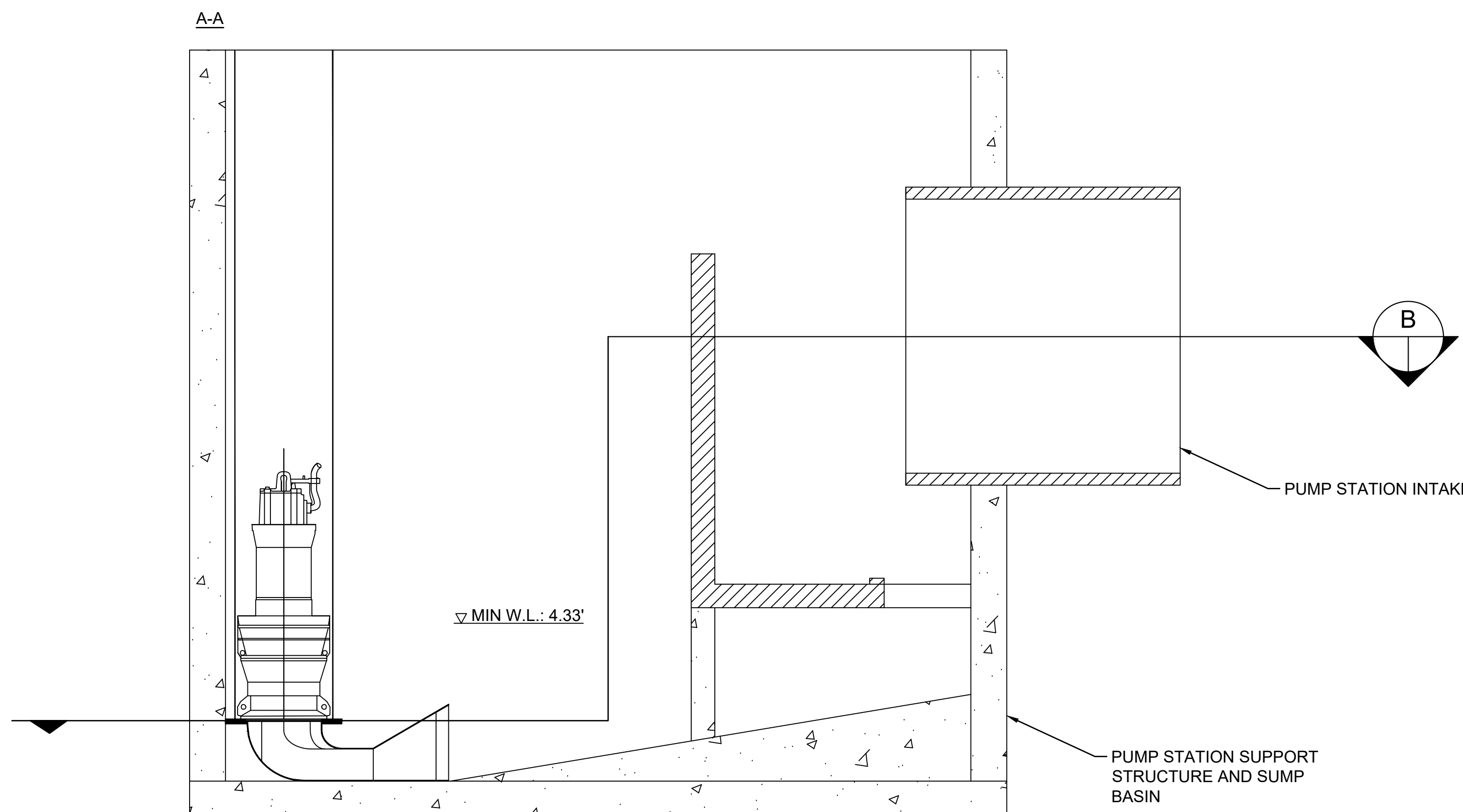
SECTION VIEW A-A
